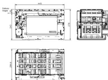
Rear Service Dimensions (mm)
