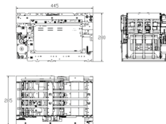
Front Service Dimensions (mm)
