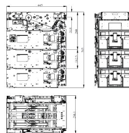
Rear Service Dimensions (mm)
