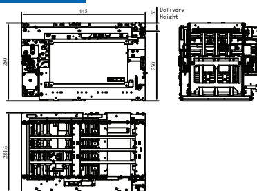
Front Service Dimensions (mm)
