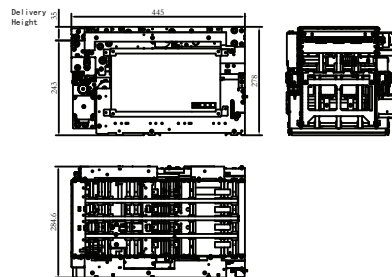
Rear Service Dimensions (mm)
